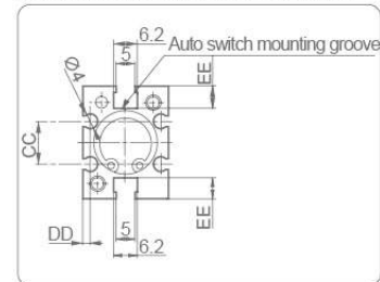
XHZ-□□ Auto Switch Mounting Groove Dimensions
